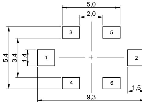
Pattern Dimensions
