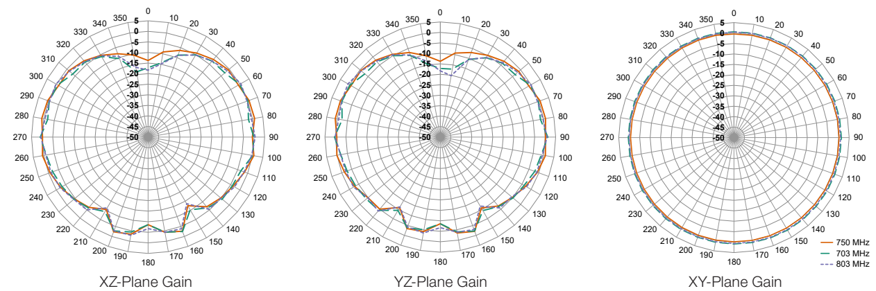
Figure8. Radiation Patterns for PW LTE Band 28 Antenna
