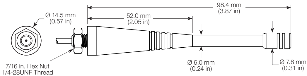
Figure 6. PW LTE Band 28 Antenna Dimensions
