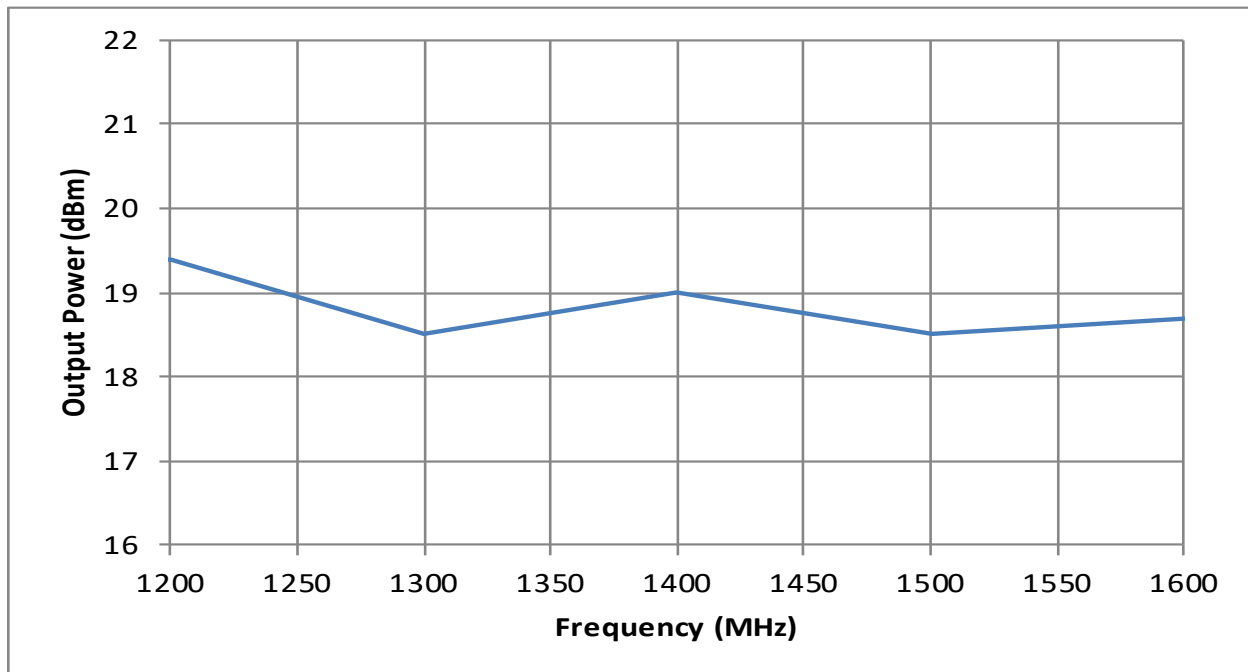
Output Power at 1 dB Compression Point
