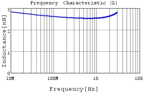
LQG15WZ2N6C02 L
