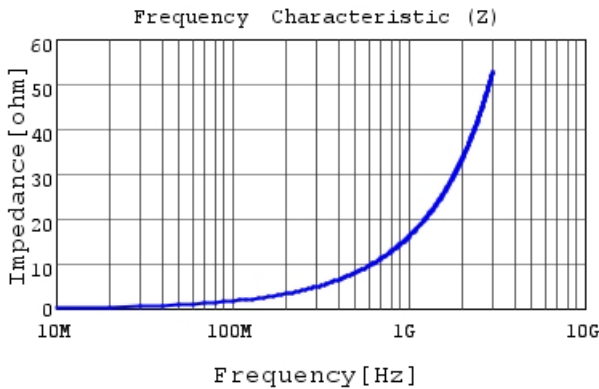
LQG15WZ2N6C02 |Z|
