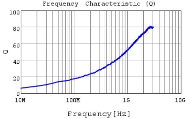
LQG15WZ2N6C02 Q
