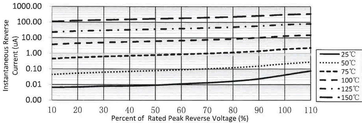
Figure 4. Typical Reverse Characteristics
