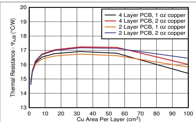
Figure 8-3. \psi_{JB} vs Copper Area 2s2p DCY Package
