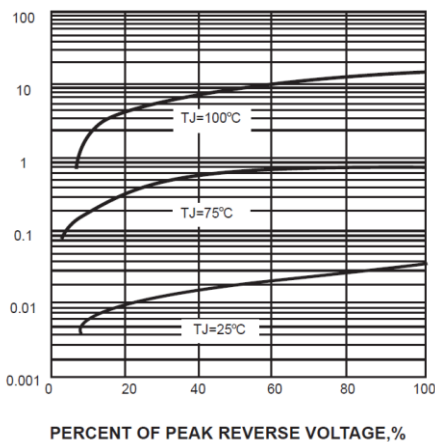
FIG. 4-TYPICAL REVERSE CHARACTERISTICS
