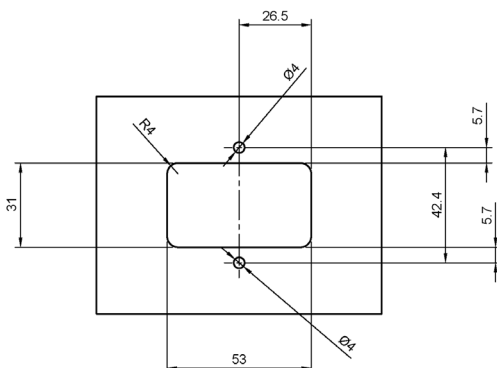
Panel cut-out recommendation (mm)
