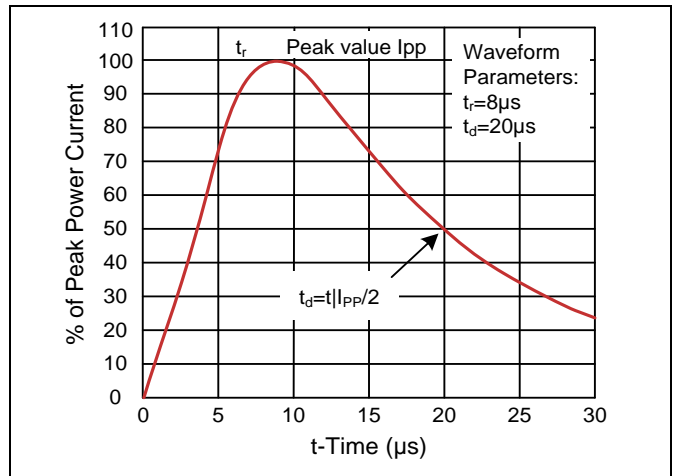
Figure 2. Pulse Waveforms
