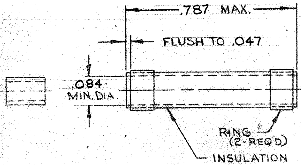
BUSHING
