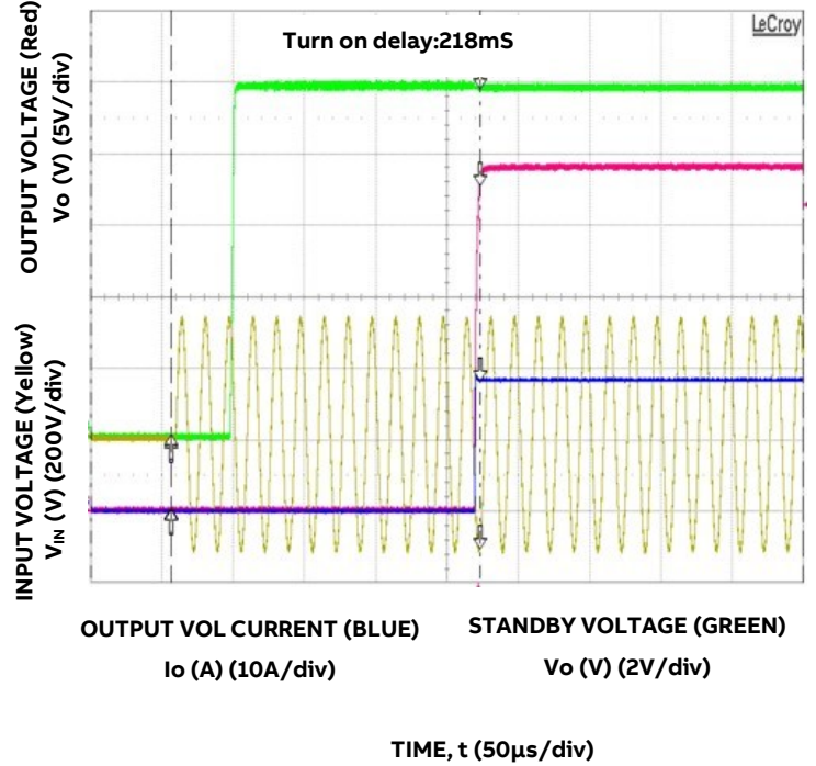
Figure 5. Typical Start-up ( V_{IN} = 230\text{V} , Full Load)
