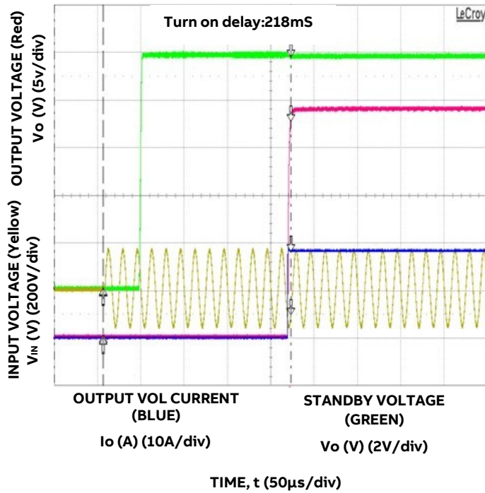
Figure 4. Typical Start-up ( V_{IN} = 115\text{Vac} , Full Load)
