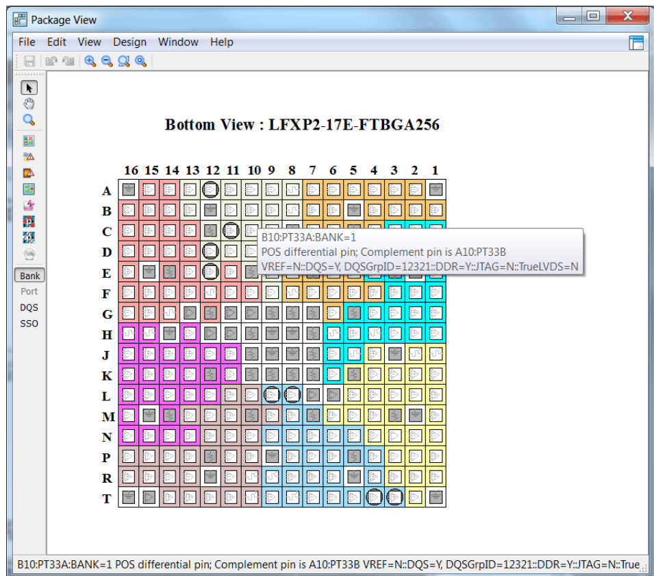
Figure 87: Package View
