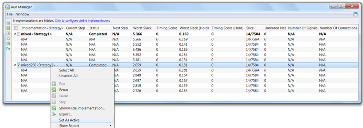
Figure 127: Run Manager
