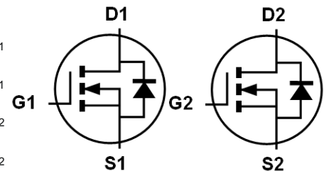
Equivalent Circuit
