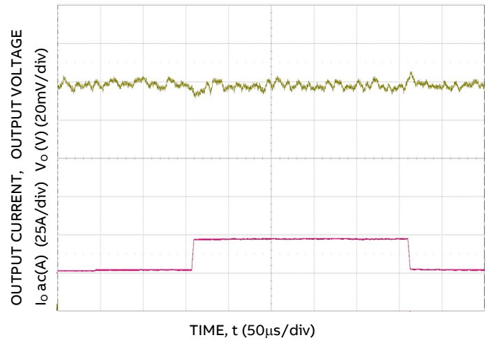
Figure 22. Trans. Resp. to 10\text{A}/\mu\text{s} Load Change from 25% to 75% at 12V_{IN} , C_o = 4 \times 0.047\mu\text{F} + 4 \times 0.1\mu\text{F} + 15 \times 22\mu\text{F} + 73 \times 47\mu\text{F} + 6 \times 470\mu\text{F} polymer
