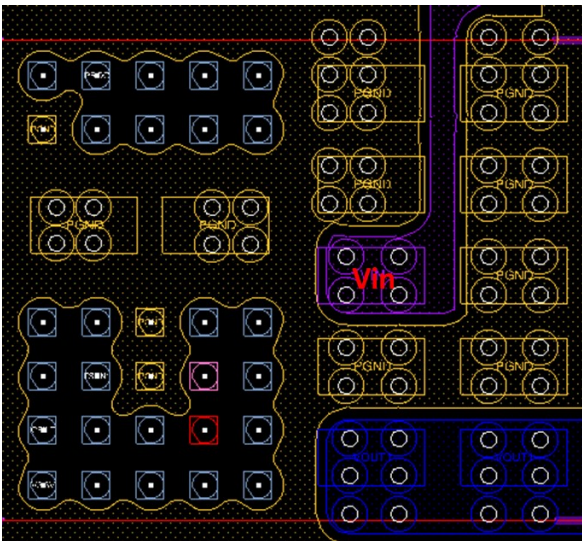
Figure 29. Example of Pad Layout with Vias.
