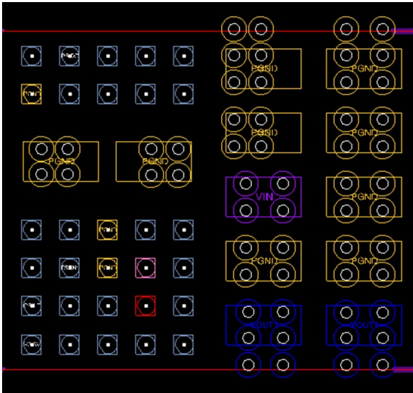
Figure 28. Example of Pad Layout with Vias.
