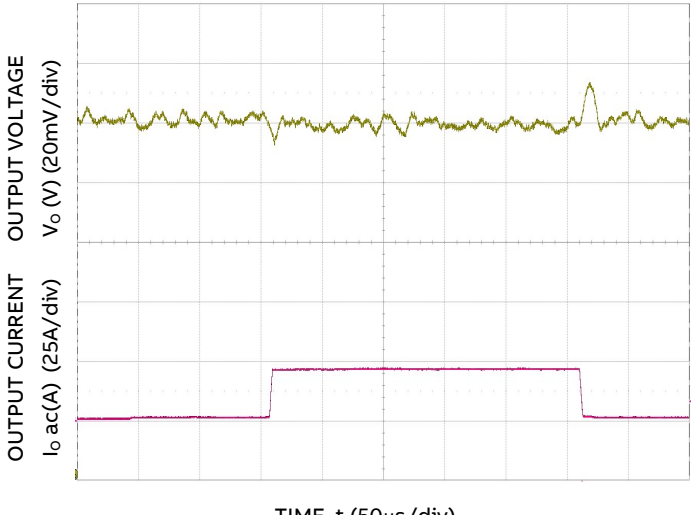
Figure 4. Trans. Resp. to 10A/µs Load Change from 25% to 75% at 12VIN, C_o=4 \times 0.047\mu\text{F} + 4 \times 0.1\mu\text{F} + 15 \times 22\mu\text{F} + 73 \times 47\mu\text{F} + 6 \times 470\mu\text{F} polymer
