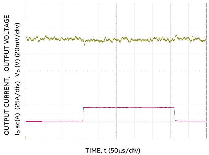
Figure 16. Trans. Resp. to 10\text{A}/\mu\text{s} Load Change from 25% to 75% at 12\text{V}_{IN} , C_o = 4 \times 0.047\mu\text{F} + 4 \times 0.1\mu\text{F} + 15 \times 22\mu\text{F} + 73 \times 47\mu\text{F} + 6 \times 470\mu\text{F} polymer
