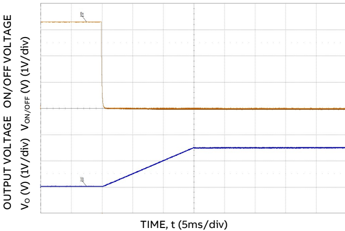
Figure 17. Typical Start-up Using On/Off Voltage ( I_o = I_{o,max} ).
