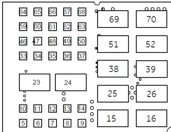
BOTTOM VIEW (ENLARGED for READABILITY)
