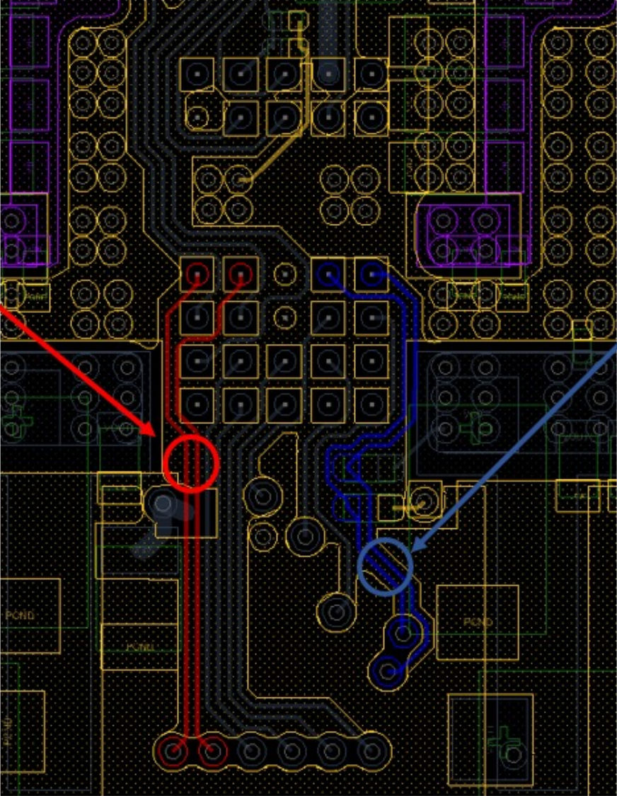
Figure 33. VSense Traces (MLX080 module shown above , applies to MLX040 as well)
