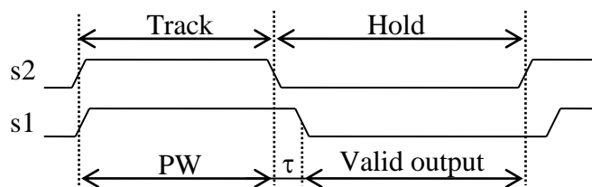
Fig. 3. Sampling Diagram
