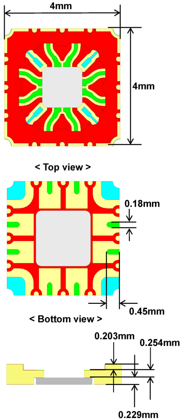
Fig. 7. CQFP 24-Pin Package Drawing (All Dimensions in mm)
