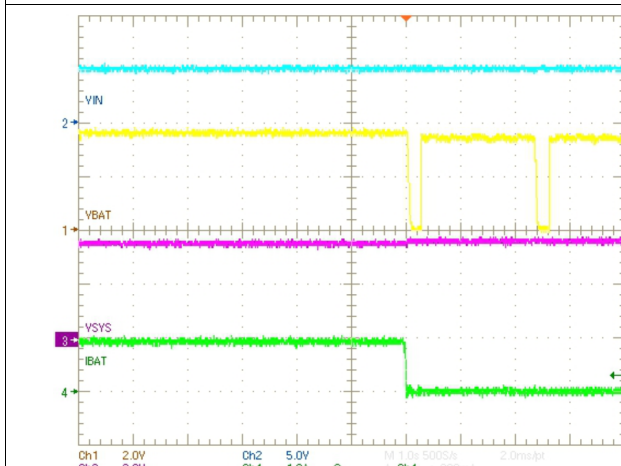
Figure 17. Battery Removal
