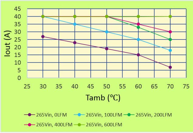
Available output current when the input voltage is 265Vac.
