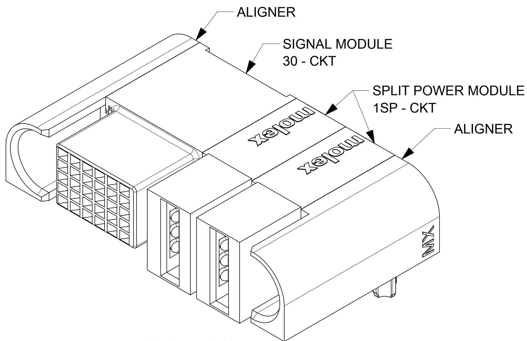
P/N: 171090-8417 (G-2SP-30S-G)
