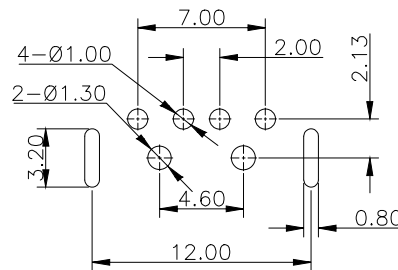
RECOMMENDED P.C.B LAYOUT (TOLERANCE:±0.05)
