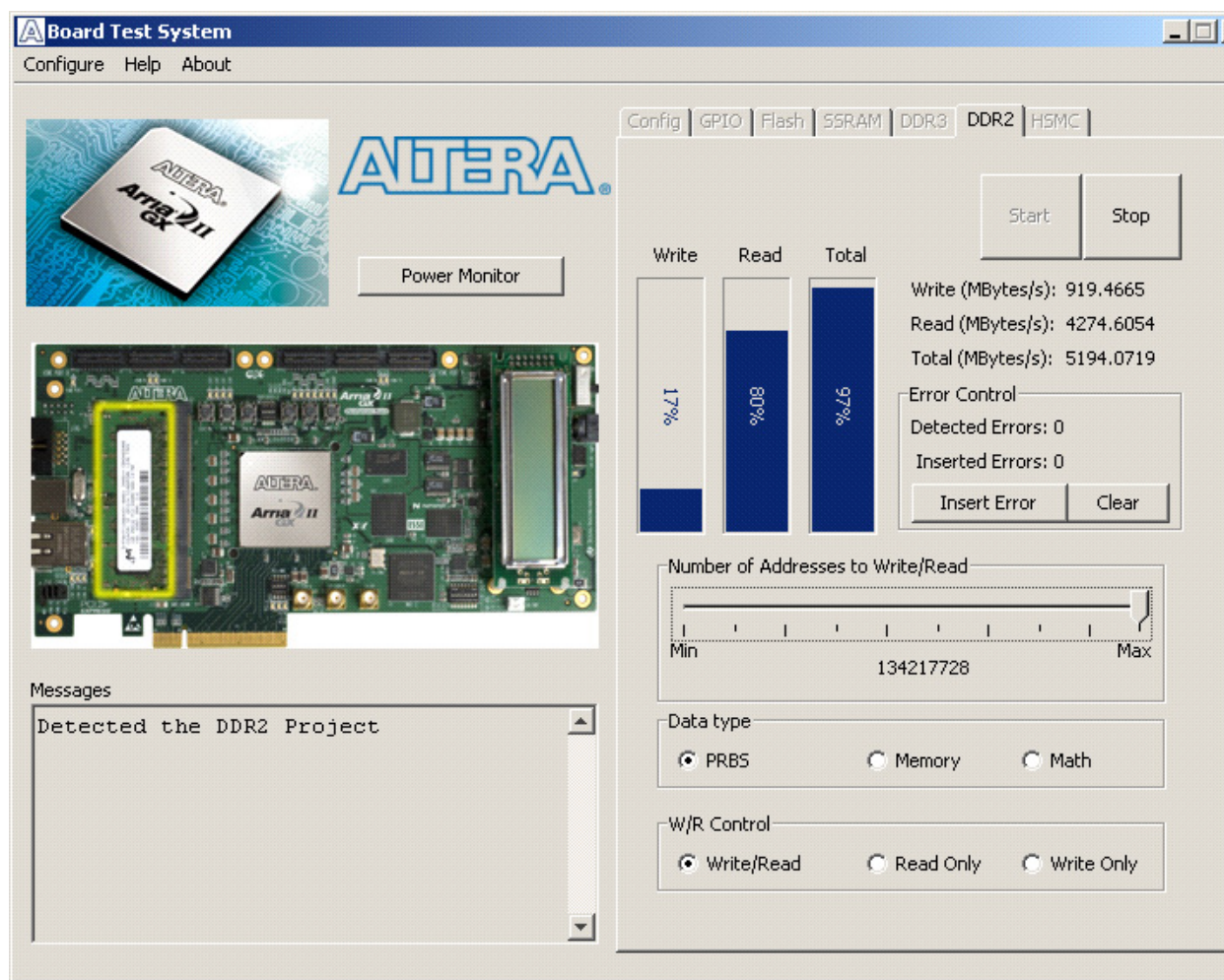
Figure 6-7. The DDR2 Tab
