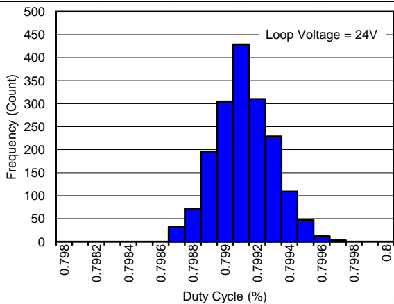
Figure 10. 0.8% Duty Cycle Distribution, PNP Mode
