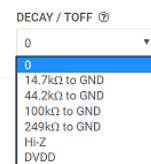
Figure 9. DRV8428E EVM GUI (Decay Mode and TOFF setting)
