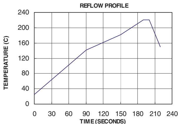
Figure 15 VPOL16A-12-SMT Reflow Profile
