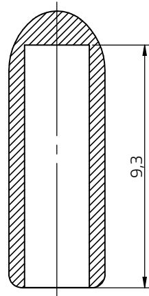
sectional drawing A-A
