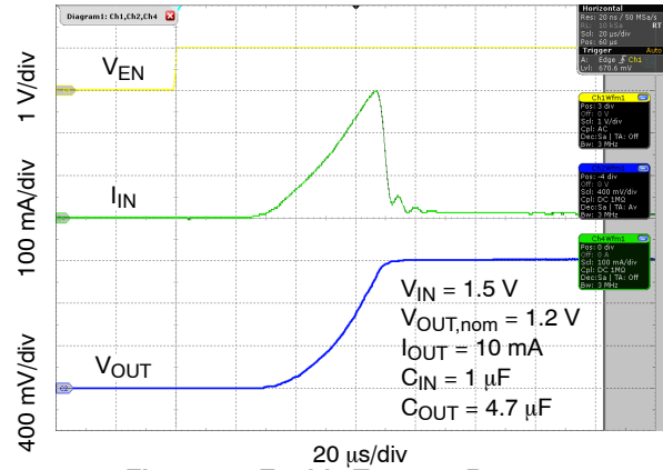
Figure 26. Enable Turn-on Response, COUT = 4.7 μF, IOUT = 10 mA
