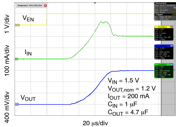
Figure 28. Enable Turn-on Response, COUT = 4.7 μF, IOUT = 200 mA
