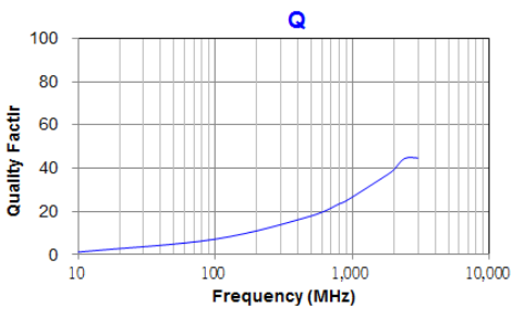
WLCM0603TN□3N9TB
