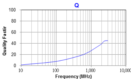
WLCM0603TN□3N5TB
