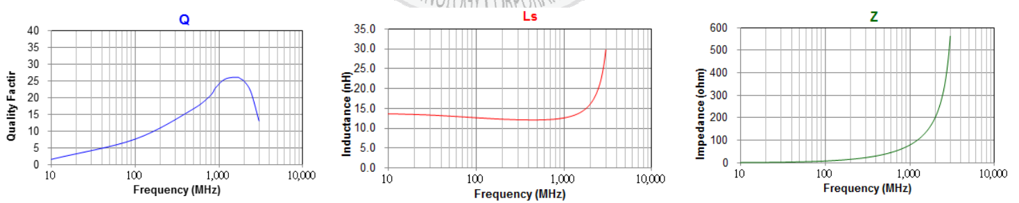
WLCM0603TN□12NTB
