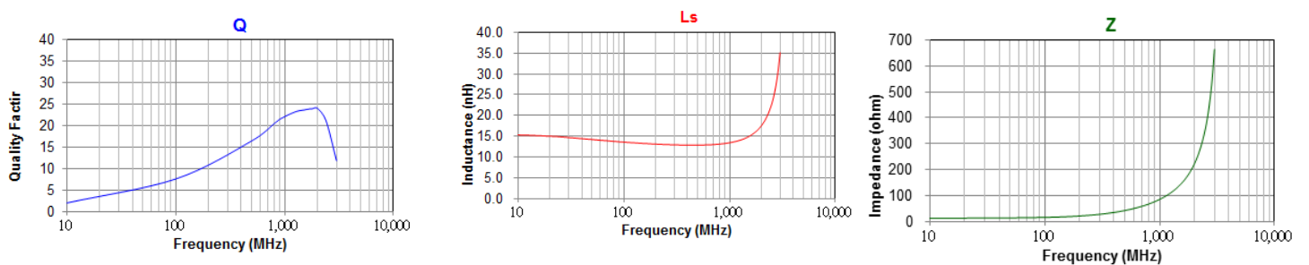
WLCM0603TN□13NTB
