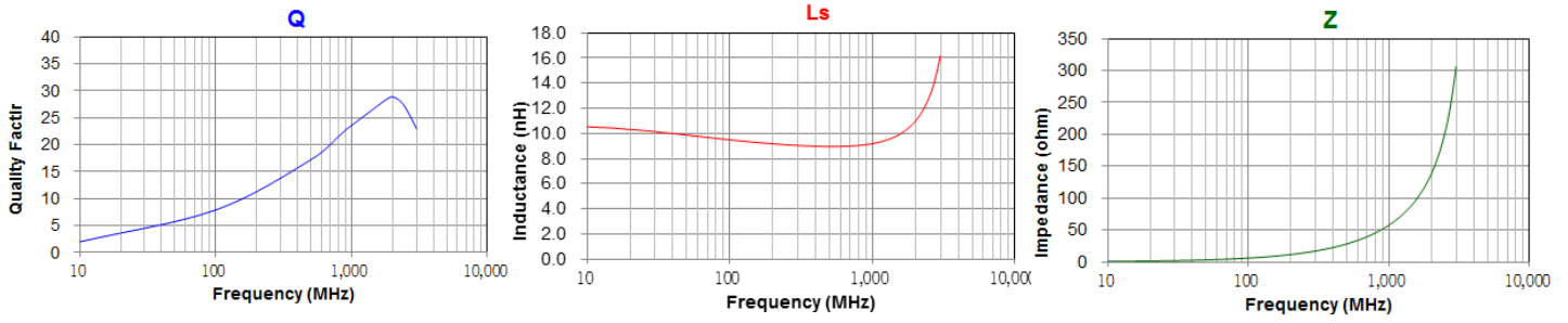
WLCM0603TN□9N1TB
