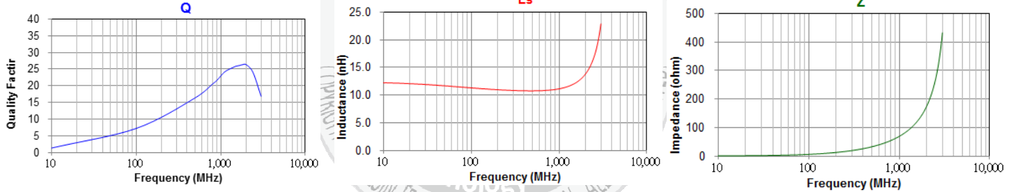
WLCM0603TN□12NTB
