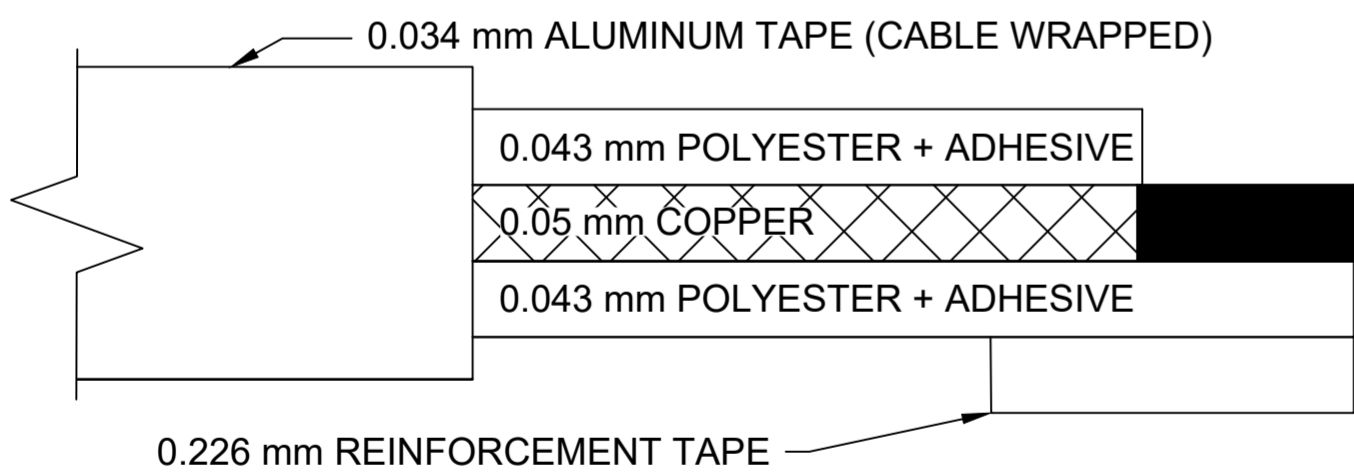
CROSS-SECTION
