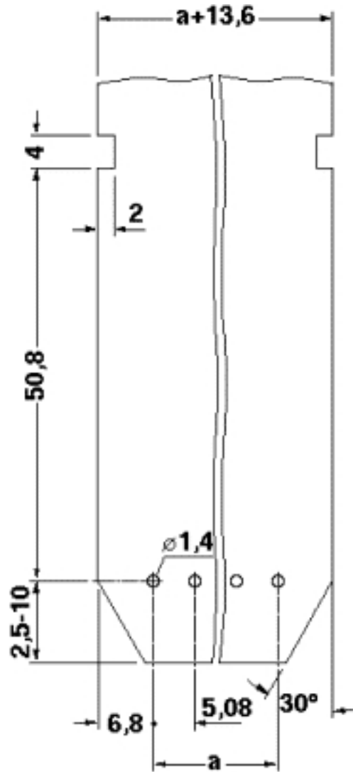
Drilling diagram
