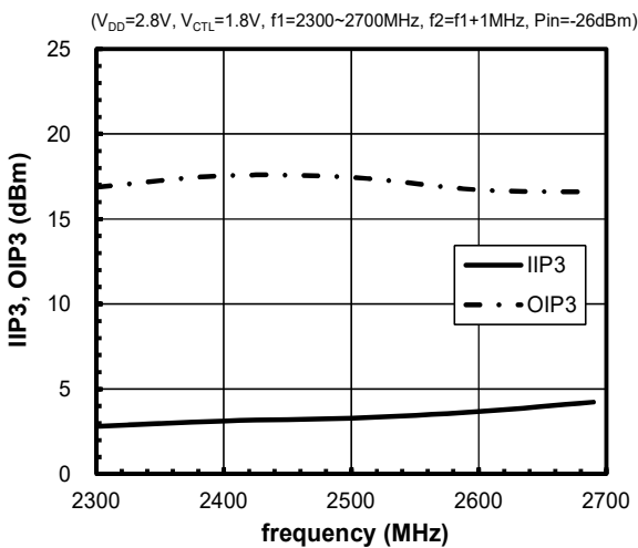
IIP3, OIP3 vs. frequency
