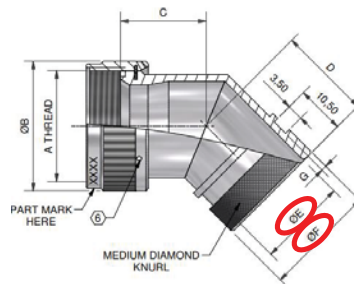
5° BACKSHELL
