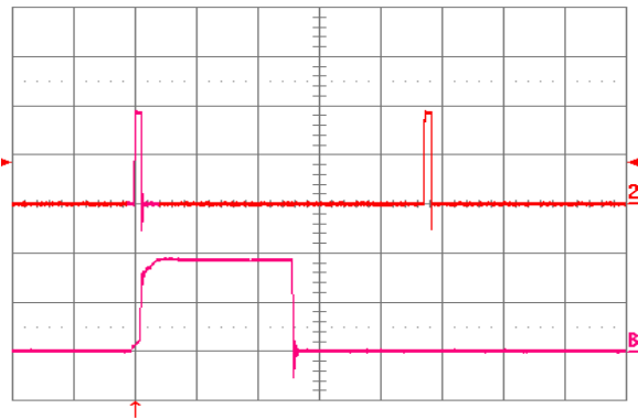
Figure 25. Load current (top trace, 20 A/div, 20 ms/div) into a 10 mΩ short circuit during restart, at V in = 24 V. Bottom trace (20 A/div, 1 ms/div) is an expansion of the on-time portion of the top trace..
