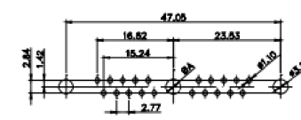
21W1 Male/Female
