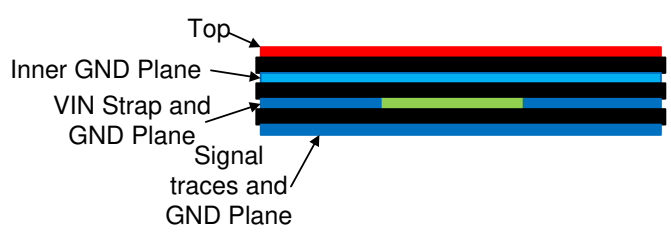
Figure 57. Example Layout
