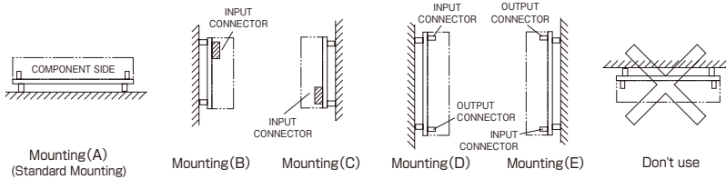
[ZWS300]
