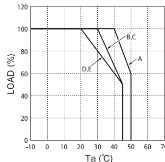
Convection Cooling Output Derating Curve (With cover)
