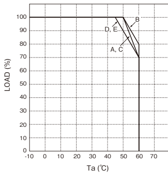
[ZWS30]
