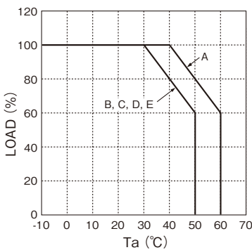
[ZWS300]
