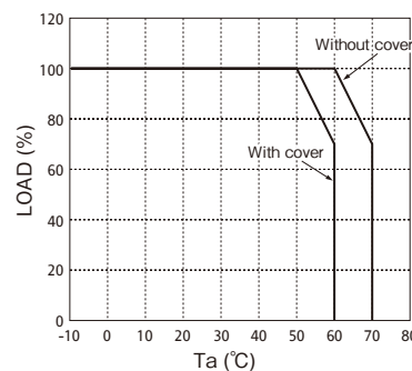
Forced Air Cooling Output Derating Curve
