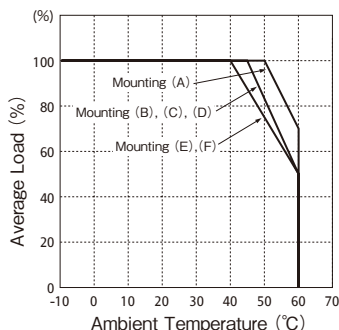
ZWS50AF Output Derating
