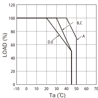
Convection Cooling Output Derating Curve (With cover)
