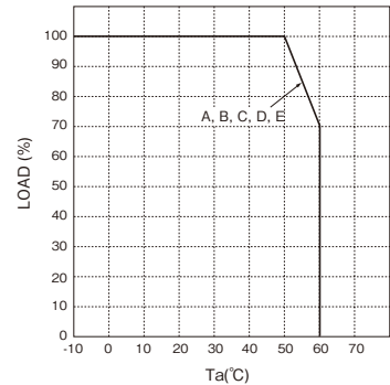
[ZWS15]
