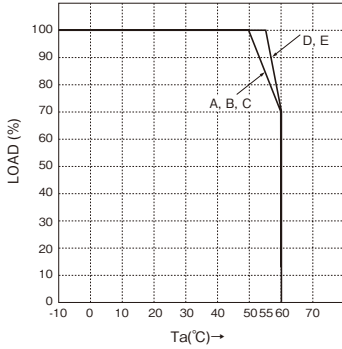
[ZWS30]
