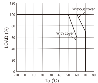
Forced Air Cooling Output Derating Curve
