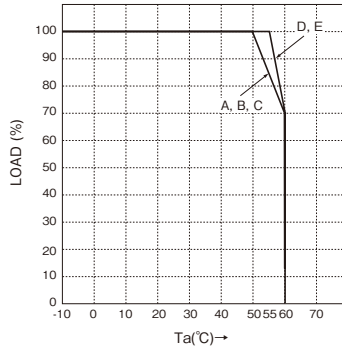
[ZWS50]
