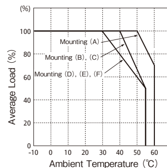
ZWS75AF
