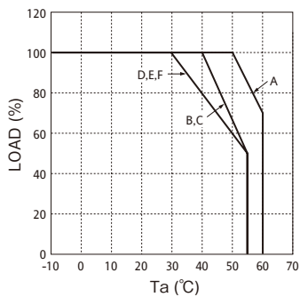
Convection Cooling Output Derating Curve (Without cover)
