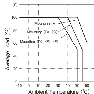
ZWS100AF Output Derating
