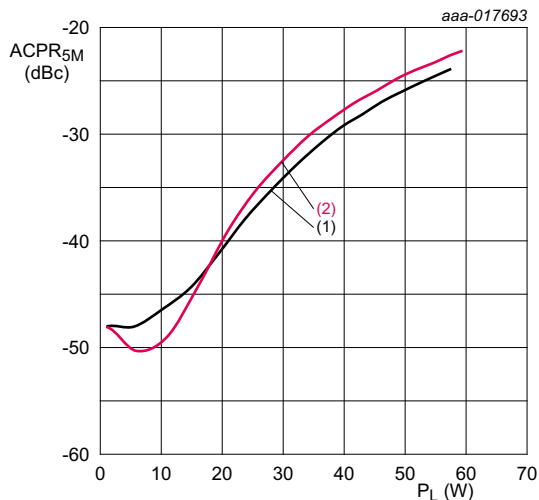
V_{DS} = 28\text{ V} ; I_{Dq} = 700\text{ mA} ; 5 MHz carrier spacing. (1) f = 1810\text{ MHz} (2) f = 1875\text{ MHz}
