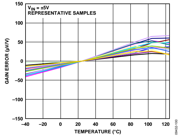
Figure 9. Gain Error vs. Temperature, V_S = \pm 5\text{ V}
