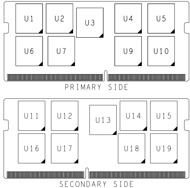
Figure 1: 260-Pin SODIMM
