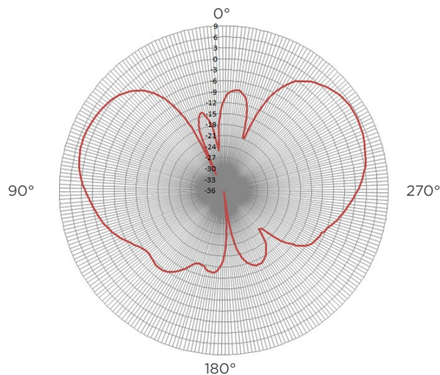
Elevation Polar Radiation Pattern 490 MHz
