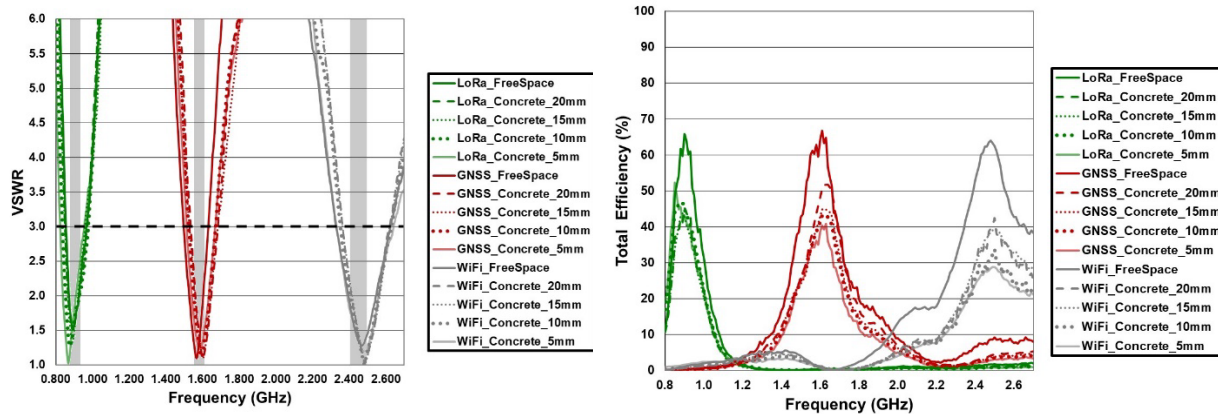
Figure 9 – VSWR and total efficiency for the different bands covered by the Evaluation Board from Figure 1 and considering the presence of concrete. The matching network used is always the same like the case 90mm x 50mm in free-space Figure 4 and Table 1.
