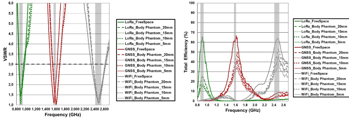
Figure 14 – VSWR and total efficiency for the different bands covered by the evaluation board from Figure 1 and considering the presence of body phantom. The matching network used is always the same like the case 90mm x 50mm in free-space Figure 4 and Table 1.
