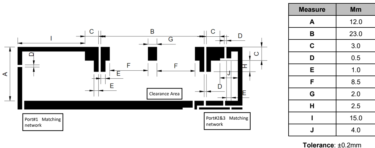
Figure 7 – Footprint dimensions for the NN03-310 chip antenna component.
