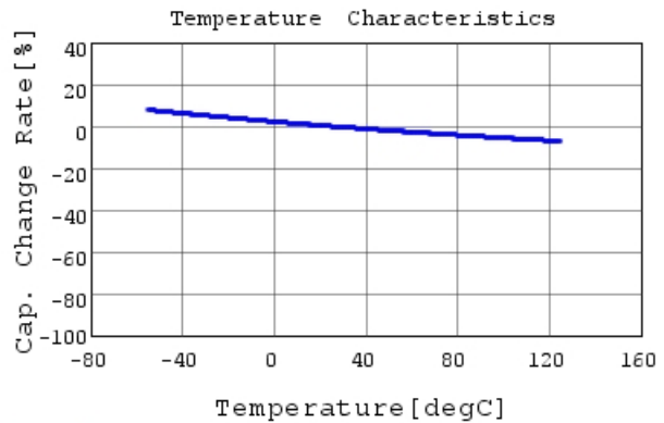
RDE7U2J153J4K1H03B C-Temp. capchange, DC0V,
