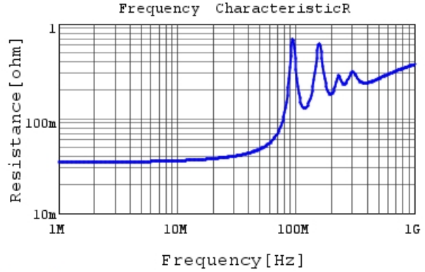
RDE7U2J153J4K1H03B R DC0V, 25degC
