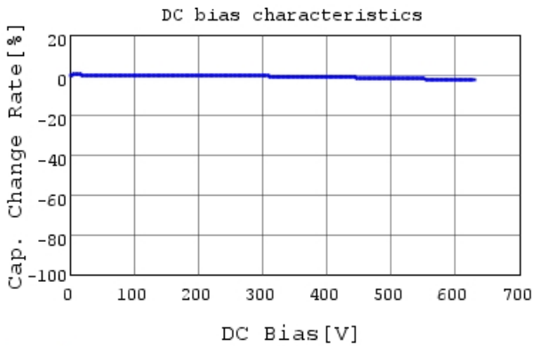
RDE7U2J153J4K1H03B C-DC bias capchange, 25.0
