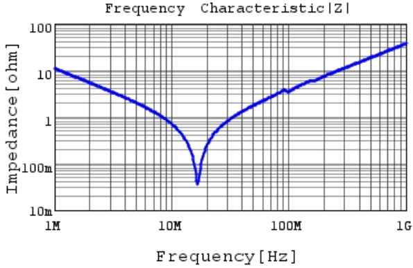
RDE7U2J153J4K1H03B |Z| DC0V, 25degC
