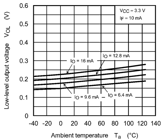
Fig. 12.2.4 V_{OL} - T_a
