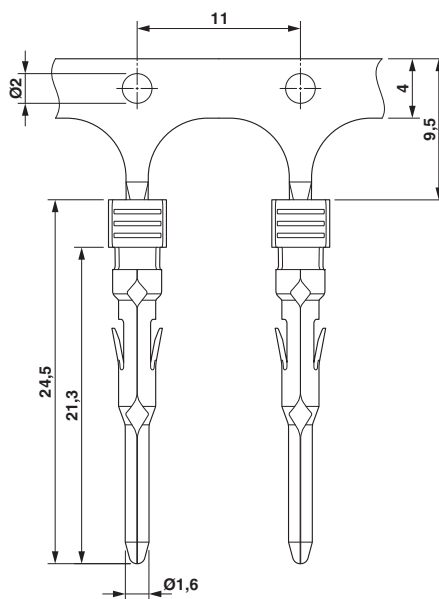
Dimensional drawing
