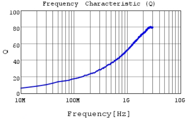
LQG15WZ2N6B02 Q
