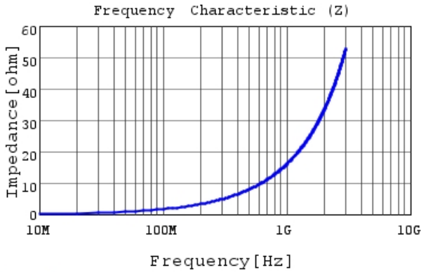
LQG15WZ2N6B02 |Z|
