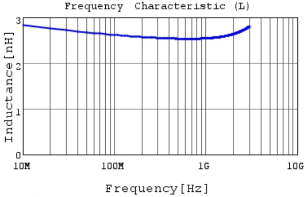
LQG15WZ2N6B02 L
