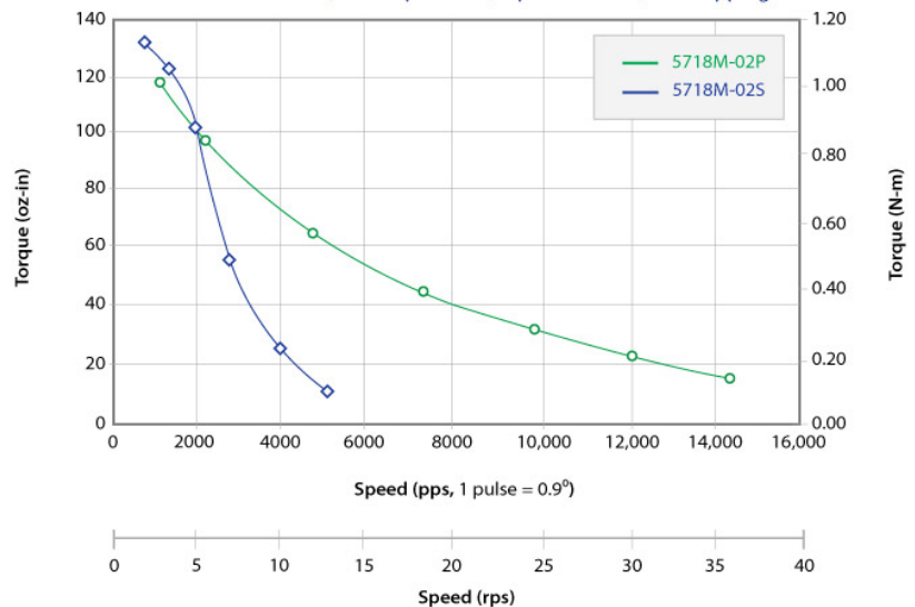
5718M-02S 24VDC, 2.1 Amps/Phase, Bipolar Series, 1/2 Stepping 5718M-02P 24VDC, 4.2 Amps/Phase, Bipolar Parallel, 1/2 Stepping
