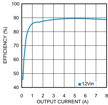
Figure 50. Efficiency
