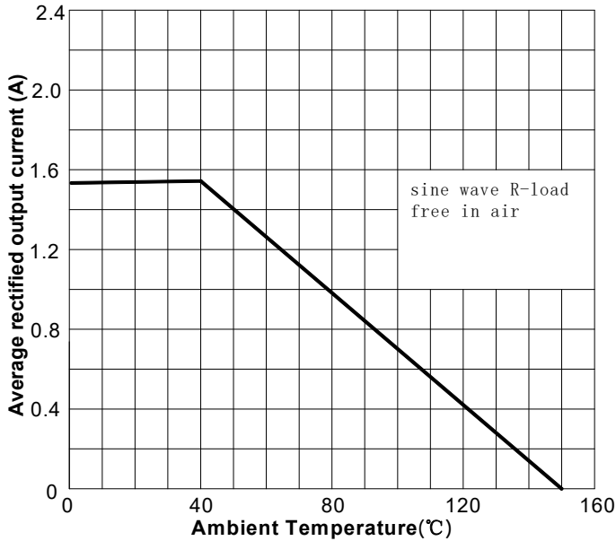
FIG1:Io-Ta Curve
