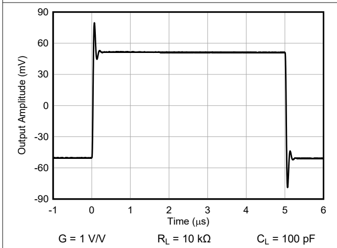
Figure 7-47. Small-Signal Response for G = 1\text{ V/V}
