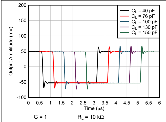
Figure 7-45. Small-Signal Response with different Output Capacitors G = 1\text{ V/V}
