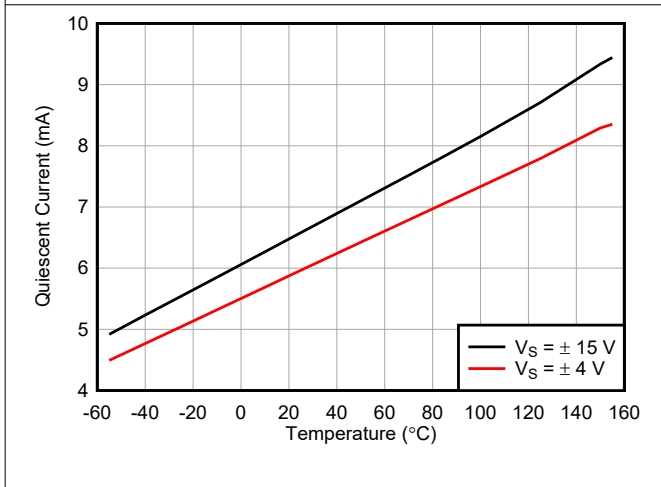
Figure 7-33. Quiescent Current vs Temperature
