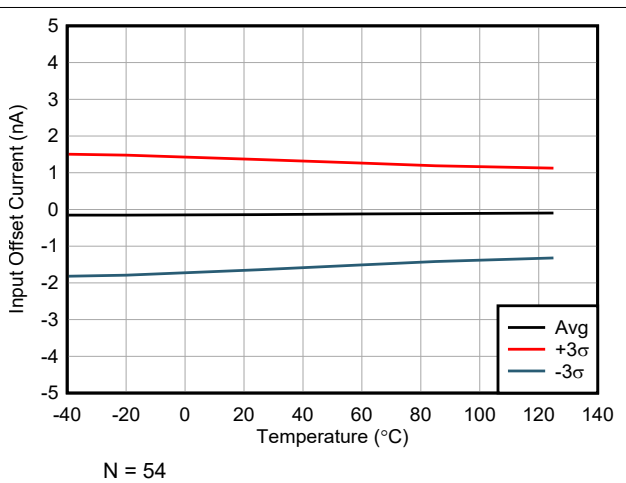
Figure 7-16. Input Offset Current vs Temperature
