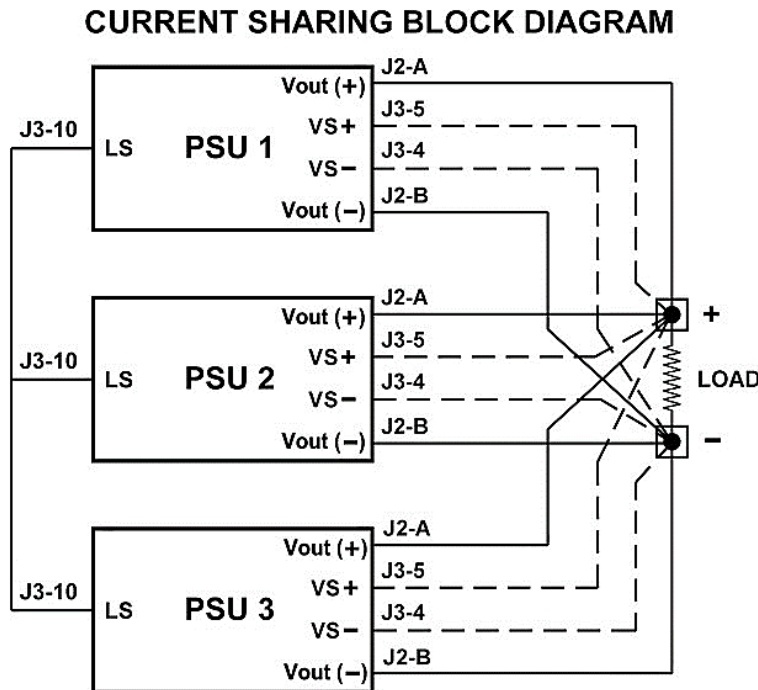
Figure 15. Current Sharing Block Diagram
