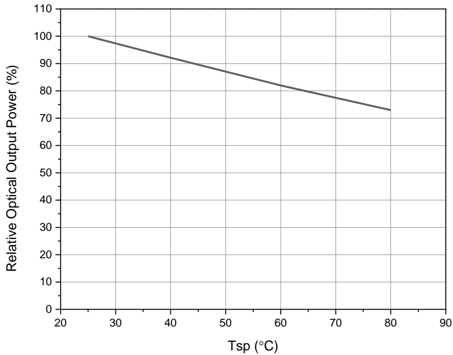
Fig 5. Relative Optical Output Power vs. Solder Point Temperature, I_F=100mA
