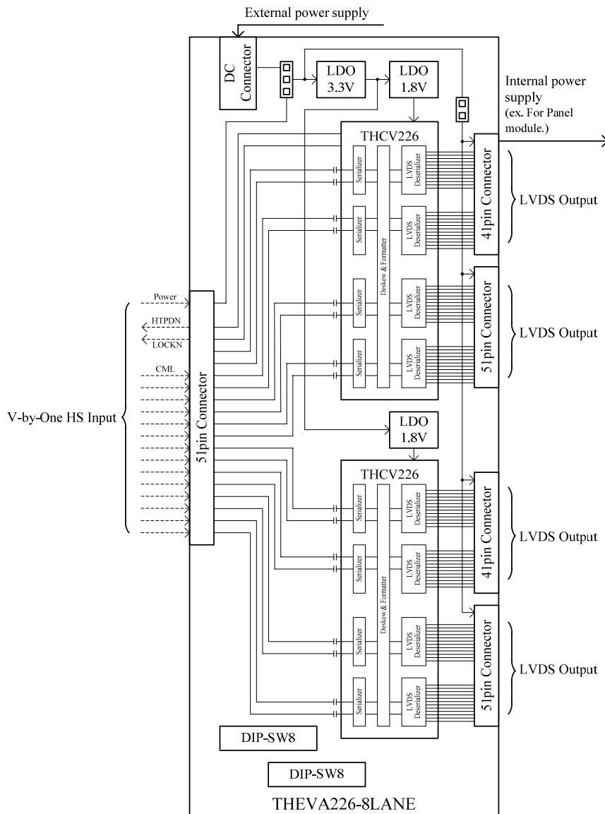
Figure2 Connection diagram
